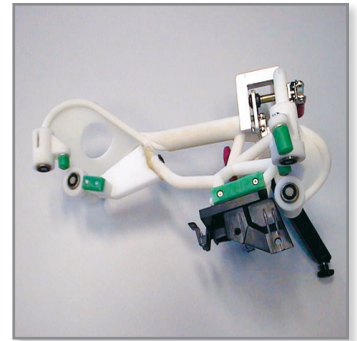
Image 4: Produced with direct digital manufacturing, this tool is used to attach bumper supports.
